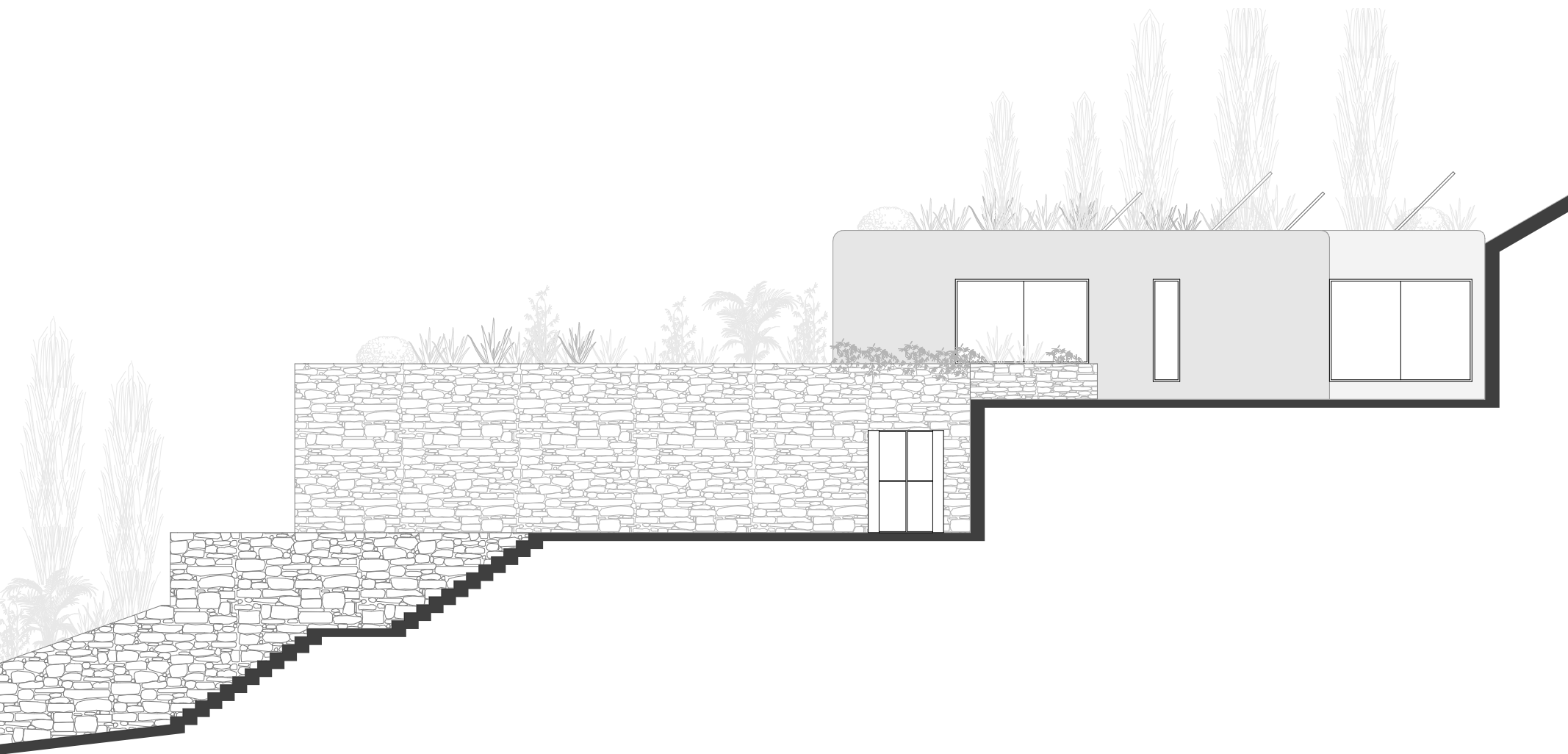
South elevation
